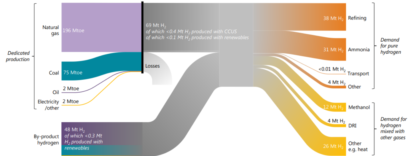
Figure 6. Today's hydrogen value chains
